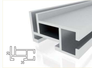
EF - FS20
